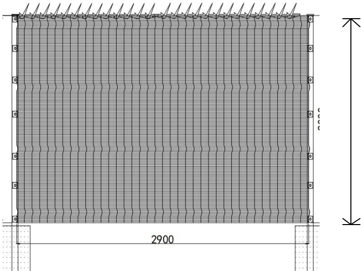
CLEAR VIEW FENCE: ELEVATION PLAN
